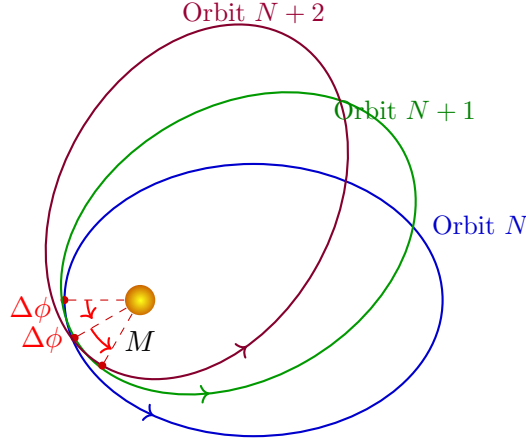
Figure 6.2: Orbital precession around a central mass.
