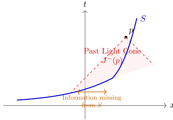
Figure 3.13: An incomplete Cauchy surface S failing to capture the full past of p .
