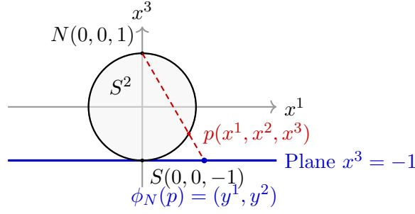
Figure 3.6: Stereographic projection of the 2-sphere ( S^2 ) from the North pole onto the South pole tangent plane, mapping S^2 \setminus \{N\} .
