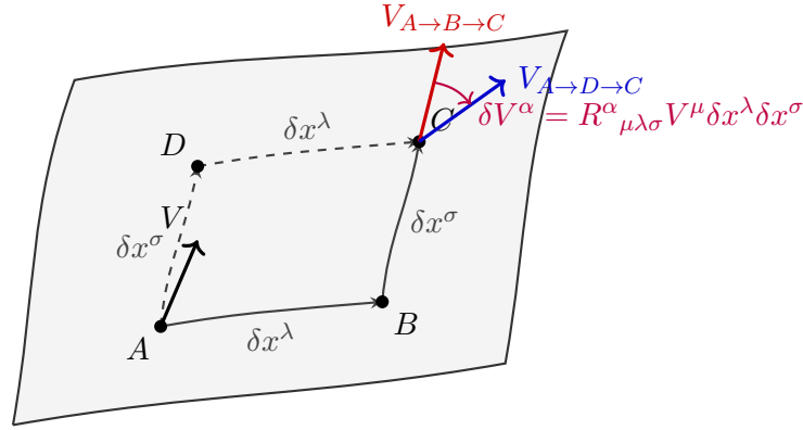
Figure 4.2: Riemann curvature defined by parallel transport around a closed loop.
