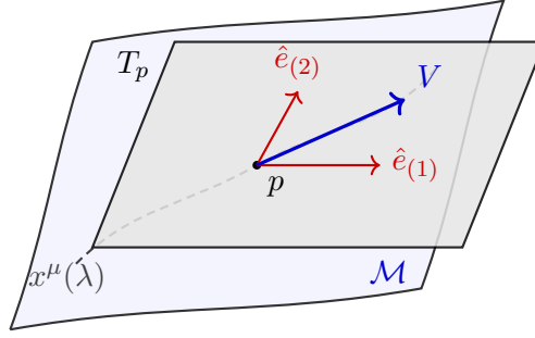
Figure 2.2: Geometric representation of a curve x^\mu(\lambda) and its tangent vector V^\mu in the local tangent space T_p of a manifold \mathcal{M} .
