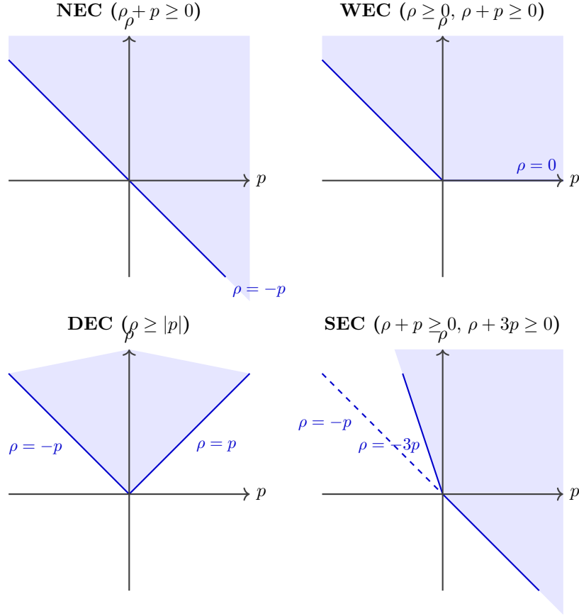
Figure 5.1: The four standard energy conditions in General Relativity.
