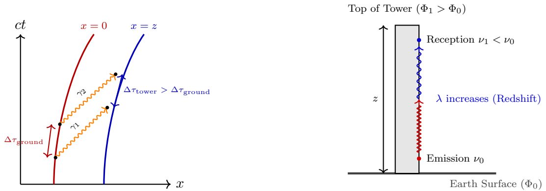
Figure 3.3: Gravitational redshift and time dilation: spacetime diagram of metric variation (left) and physical schematic of wavelength increase (right).
