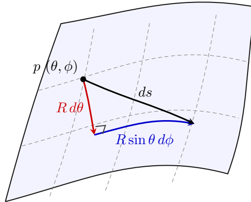
Figure 3.10: Infinitesimal line element ds on the surface of a 2-sphere.
