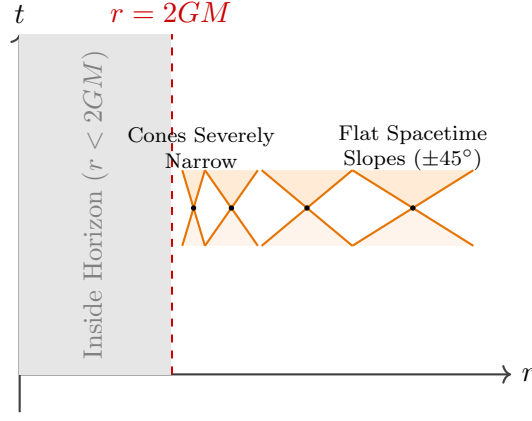
Figure 6.3: Light cones narrowing near the horizon in Schwarzschild coordinates.
