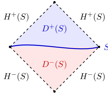
Figure 3.12: Domains of dependence and Cauchy horizons for a spacelike surface S .
