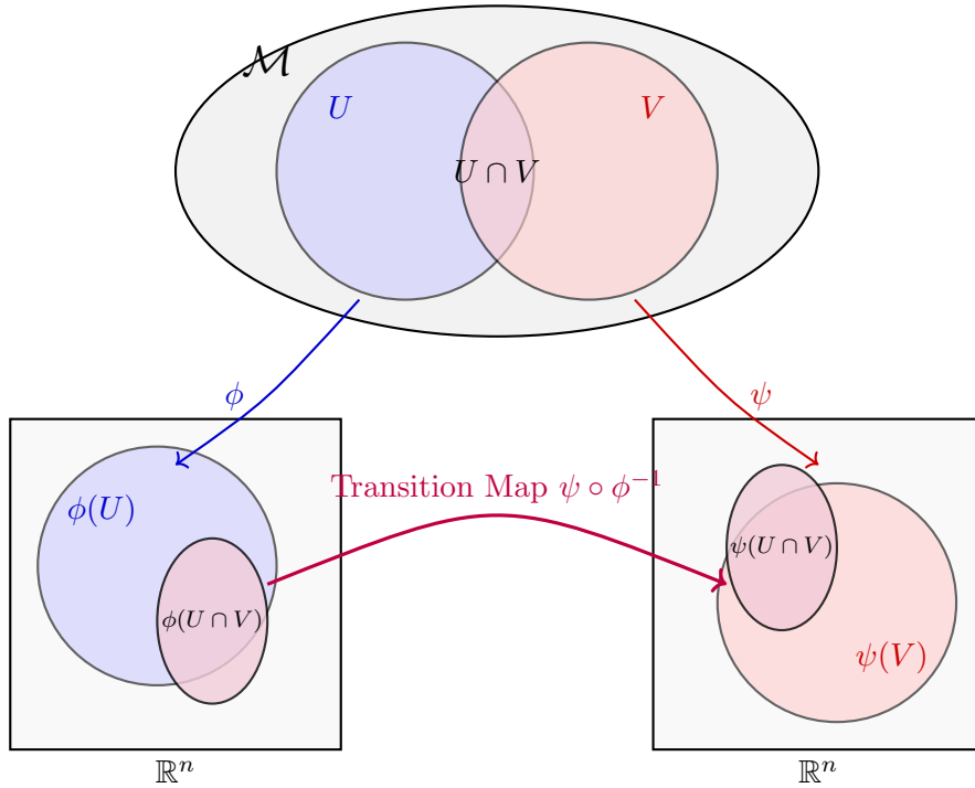
Figure 3.5: Atlas construction on a manifold \mathcal{M} : local coordinate charts \phi and \psi linked by a smooth transition map \psi \circ \phi^{-1} .
