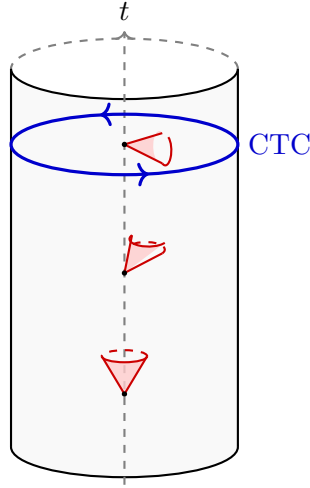
Figure 3.14: Tipping of light cones leading to the formation of a Closed Timelike Curve.
