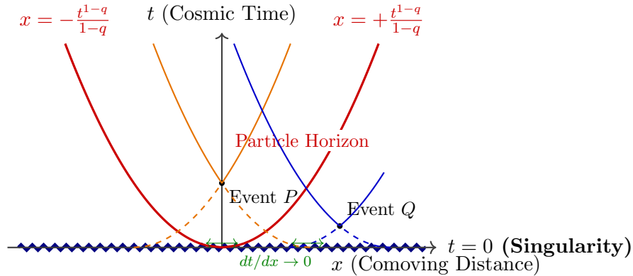
Figure 3.11: Spacetime diagram illustrating the cosmological particle horizon.
