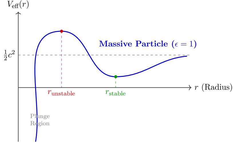
Figure 6.1: Effective potential profile for a massive particle.
