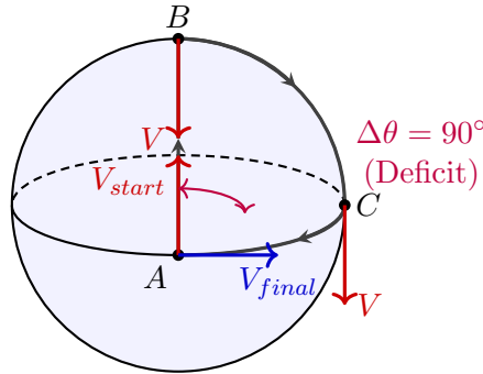
Figure 4.1: Parallel transport on a sphere resulting in a deficit angle.
