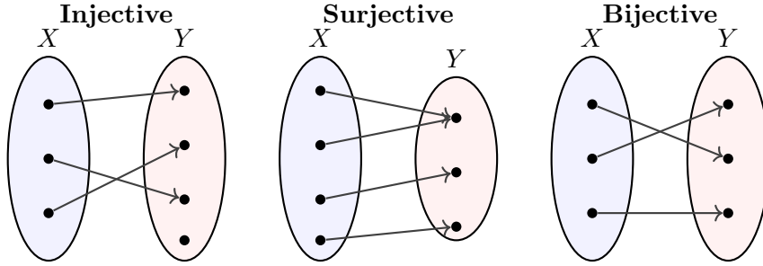
Figure 3.4: Classification of injective, surjective, and bijective mappings between sets X and Y .
