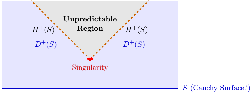
Figure 3.15: Breakdown of predictability beyond the Cauchy horizon due to a singularity.
