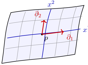
Figure 3.8: Coordinate curves and their tangent basis vectors at a point p .
