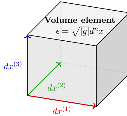
Figure 3.16: The invariant volume element in a curved space.
