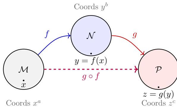
Figure 3.7: Composition of smooth maps between manifolds.
