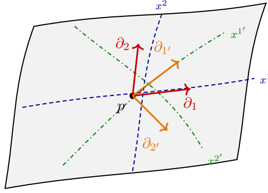
Figure 3.9: Transformation of basis vectors under a local coordinate change.
