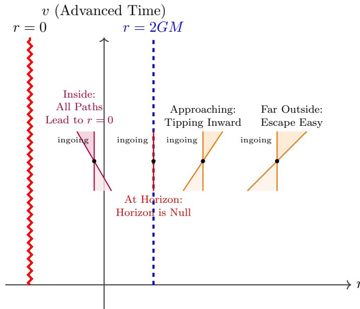
Figure 6.4: Light cones tipping inward in Eddington-Finkelstein coordinates.
