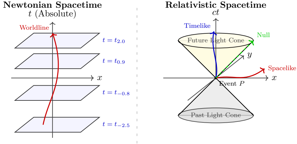
Figure 2.1: Comparison of Newtonian absolute spacetime (left) and Minkowskian causal structure (right), showing the past/future light cones of event P and its causal regions.
