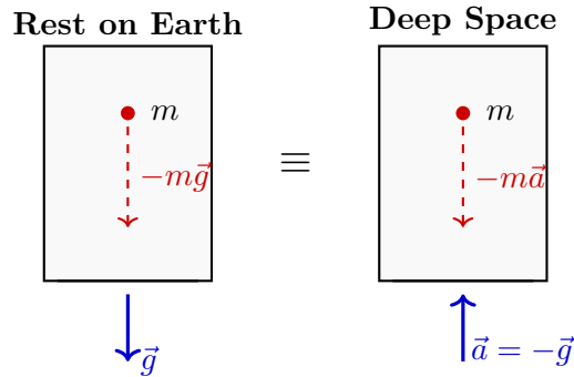
Figure 3.1: The Einstein Equivalence Principle: indistinguishability between a uniform gravitational field (left) and a uniformly accelerated frame (right).
